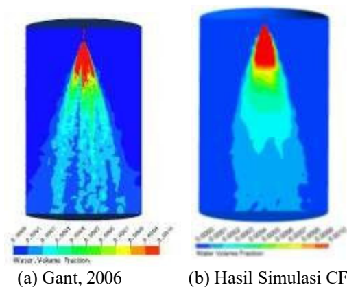
Gambar 6. Water vapour volume fraction
