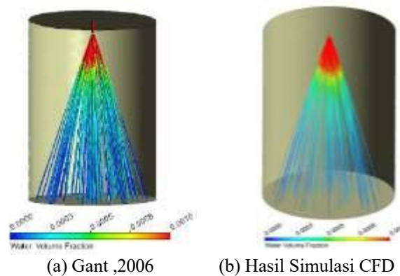
Gambar 5. Droplet trajectories
