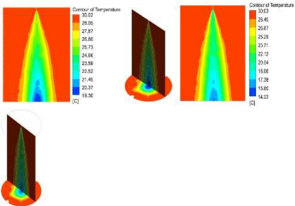
(a) Laju Aliran Massa Air 0.012 kg/s
